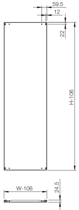
Mounting plate view
